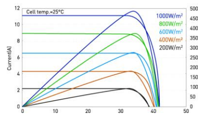
I-V/P-V Curve at Different Irradiation
